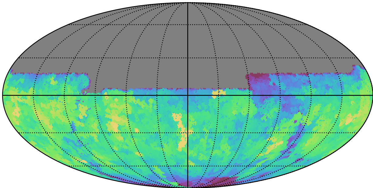
baseline_v3.2_10yrs All sky u band: Max saturation_mag
