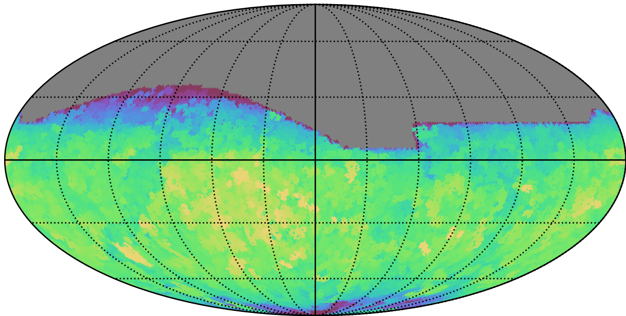
baseline_v3.2_10yrs All sky r band: Max saturation_mag
