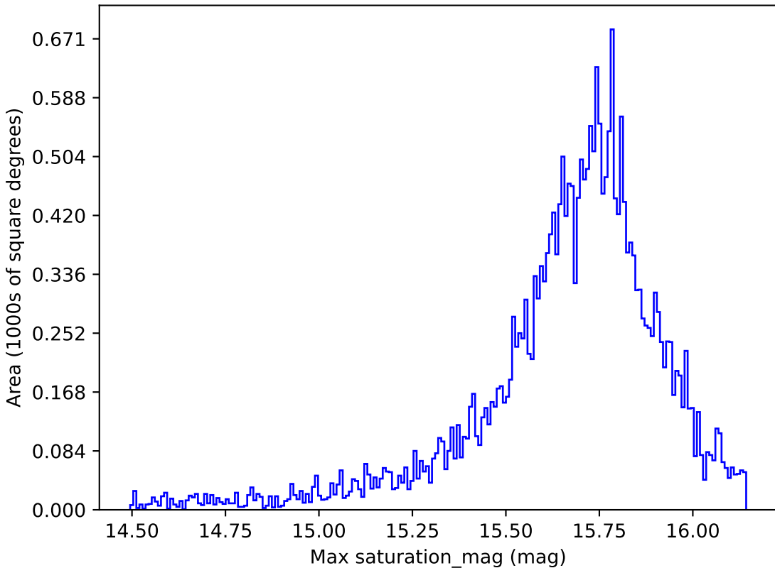
baseline_v3.2_10yrs All sky r band: Max saturation_mag
