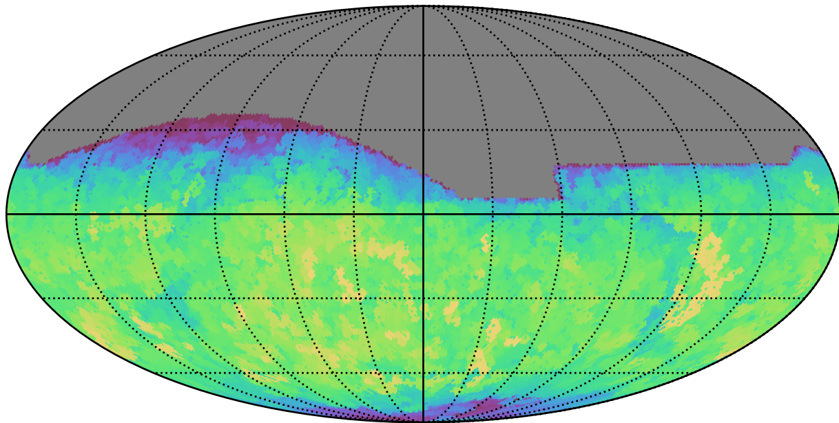
baseline_v3.2_10yrs All sky i band: Max saturation_mag
