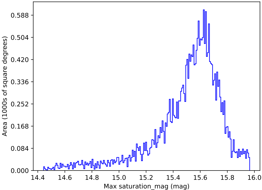
baseline_v3.2_10yrs All sky i band: Max saturation_mag
