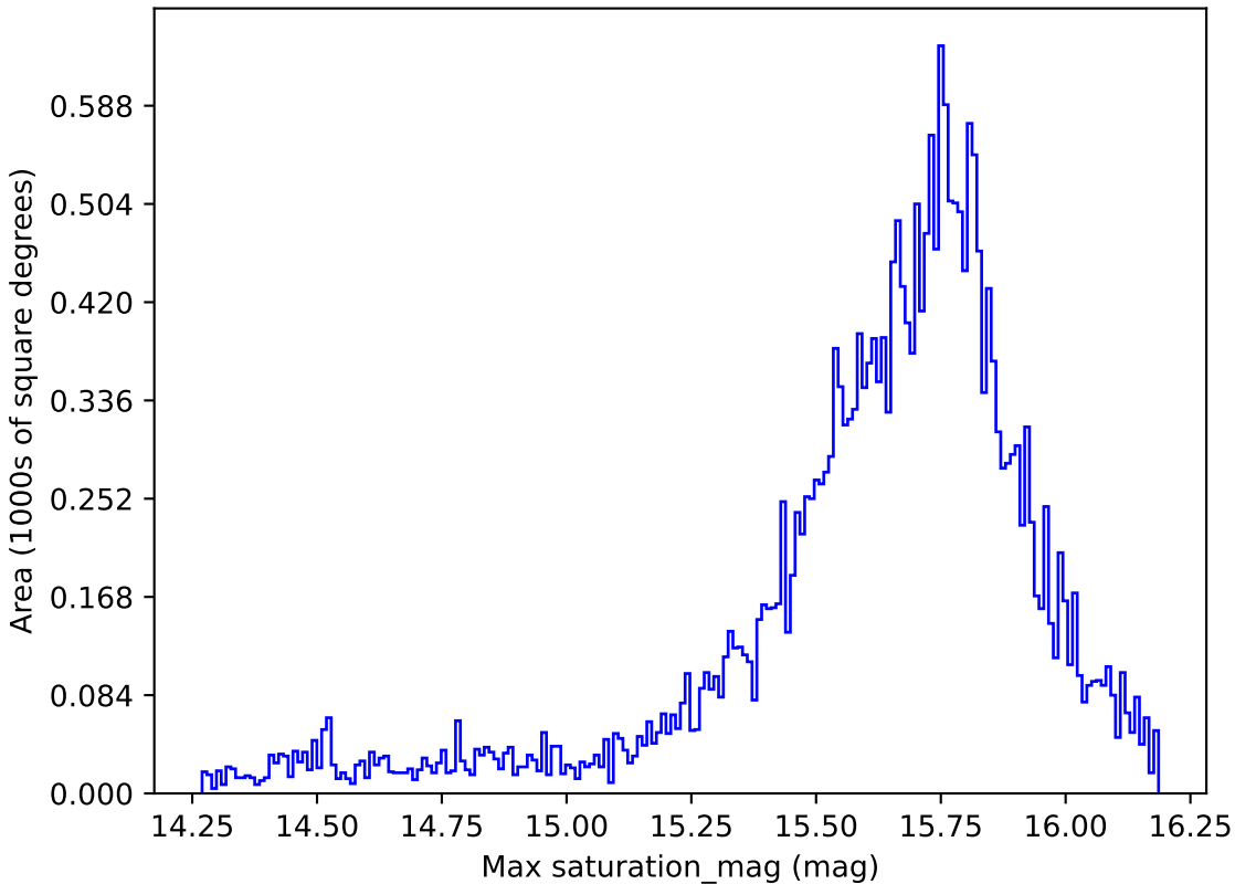
baseline_v3.2_10yrs All sky g band: Max saturation_mag
