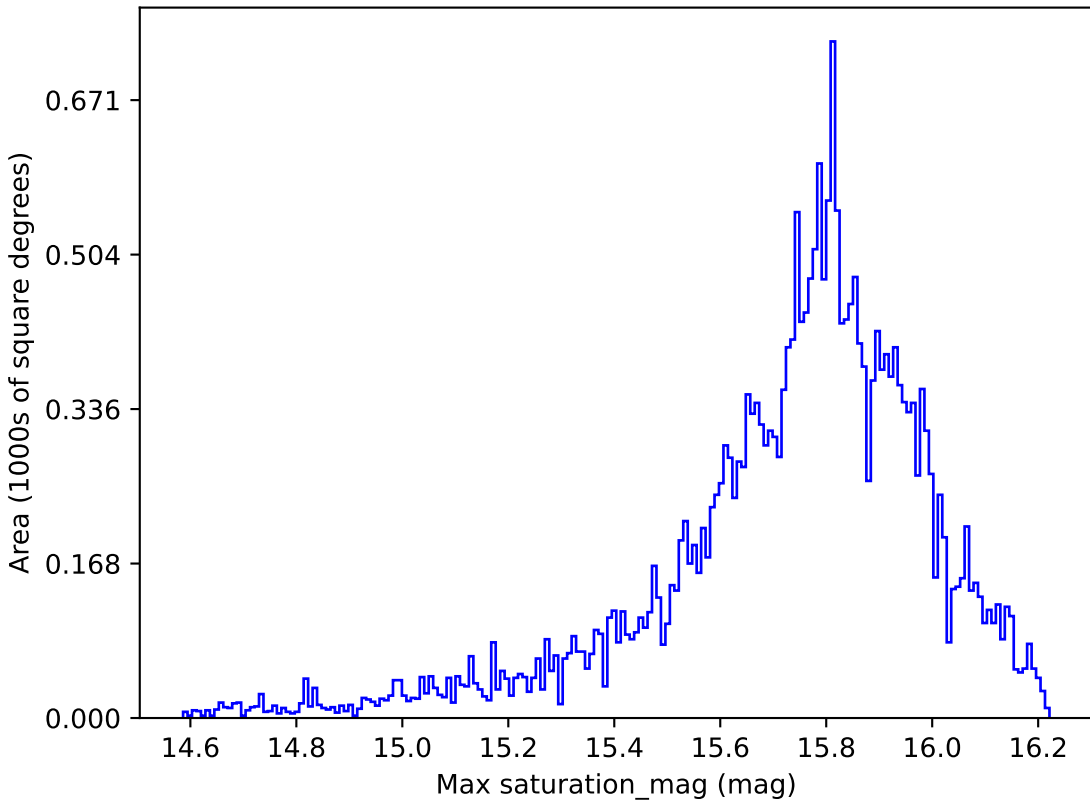
baseline_v3.2_10yrs All sky all bands: Max saturation_mag
