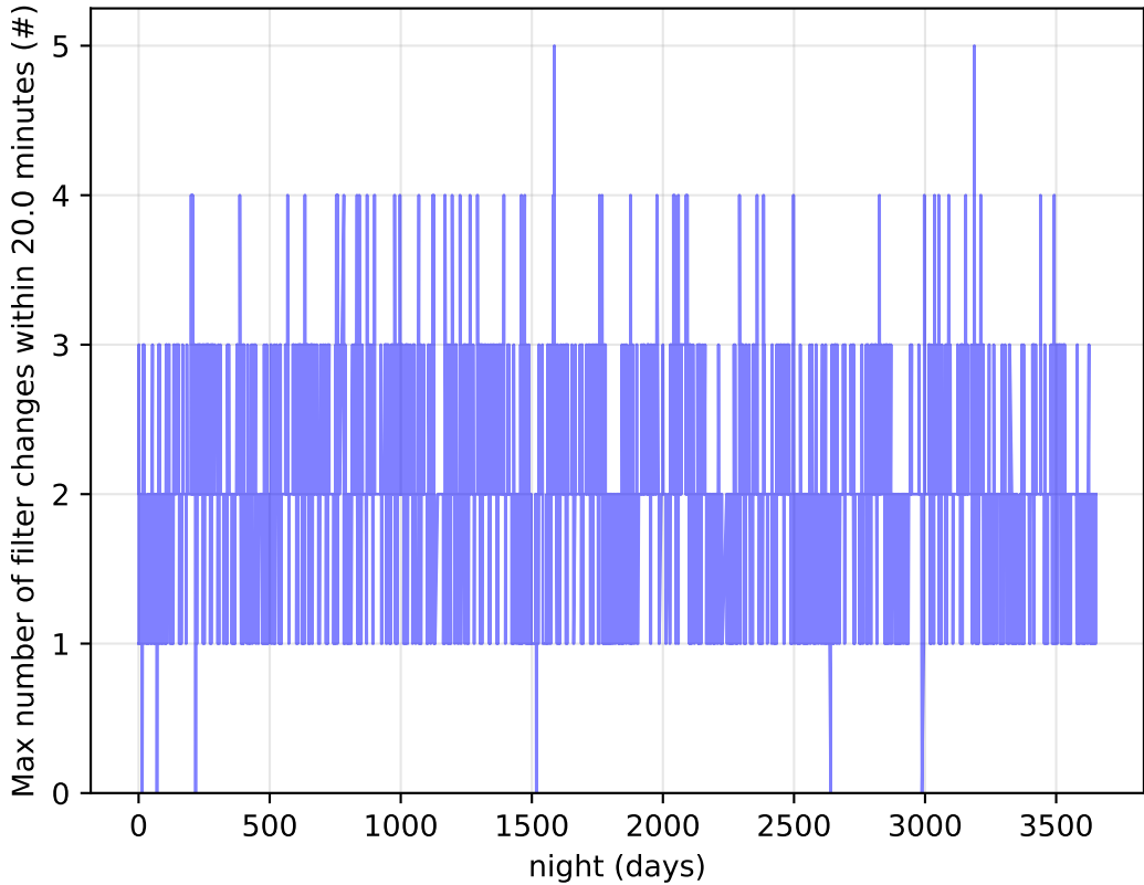
baseline_v3.2_10yrs Per Night: Max number of filter changes within 20.0 minutes
