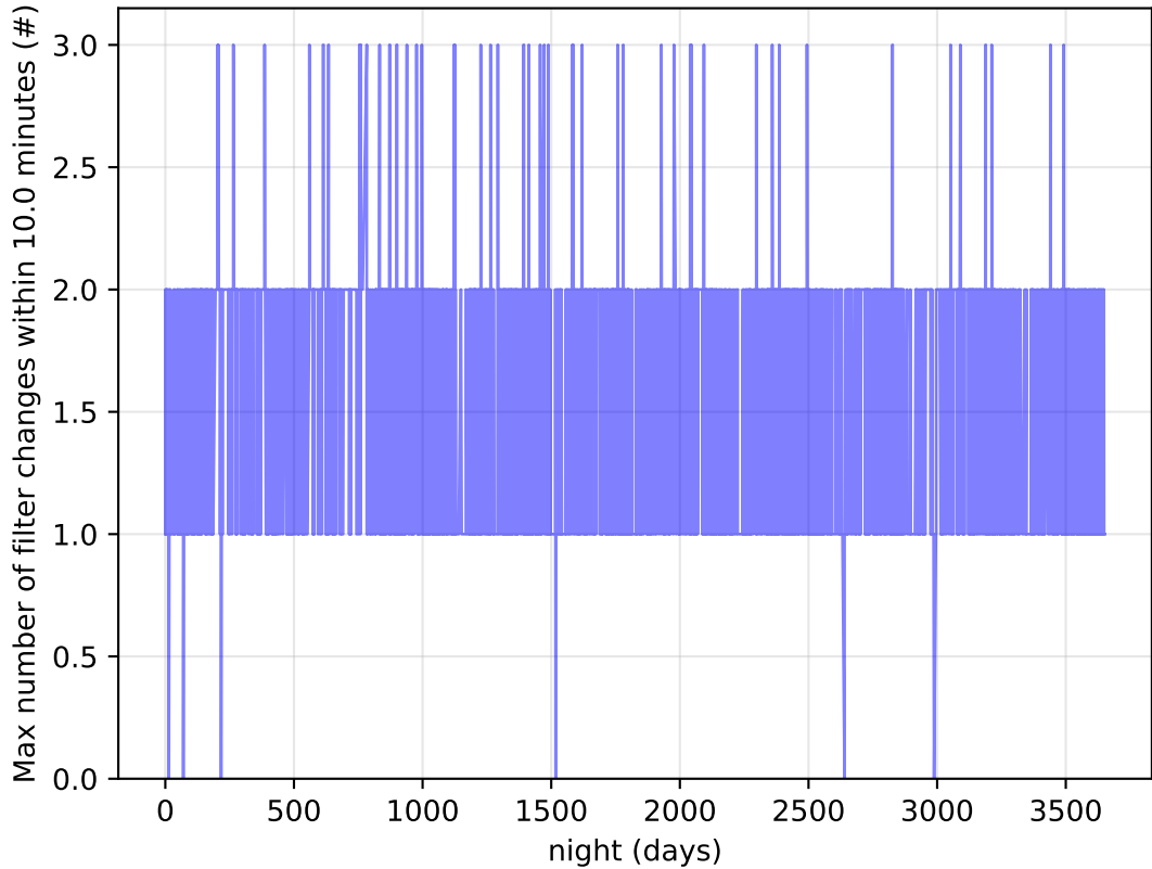
baseline_v3.2_10yrs Per Night: Max number of filter changes within 10.0 minutes
