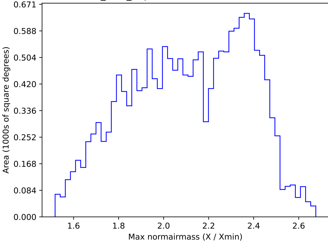
baseline_v3.2_10yrs WFD r band: Max normairmass
