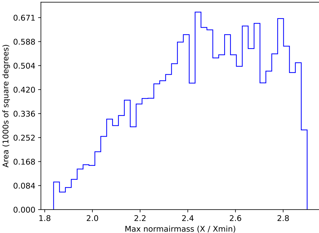
baseline_v3.2_10yrs WFD all bands: Max normairmass
