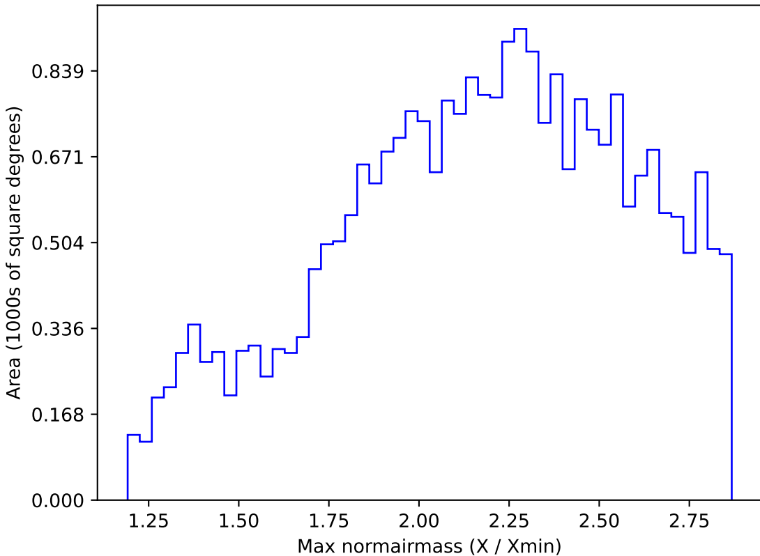
baseline_v3.2_10yrs All sky z band: Max normairmass
