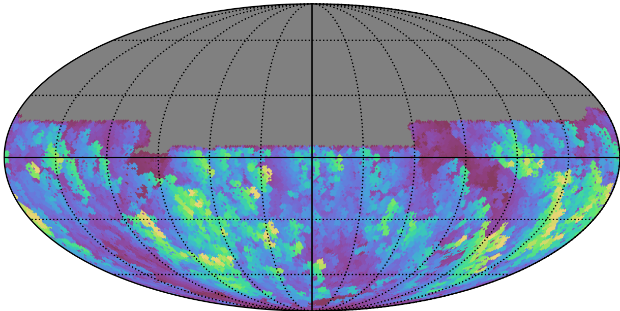
baseline_v3.2_10yrs All sky u band: Max normairmass
