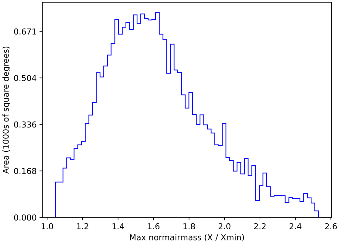
baseline_v3.2_10yrs All sky u band: Max normairmass
