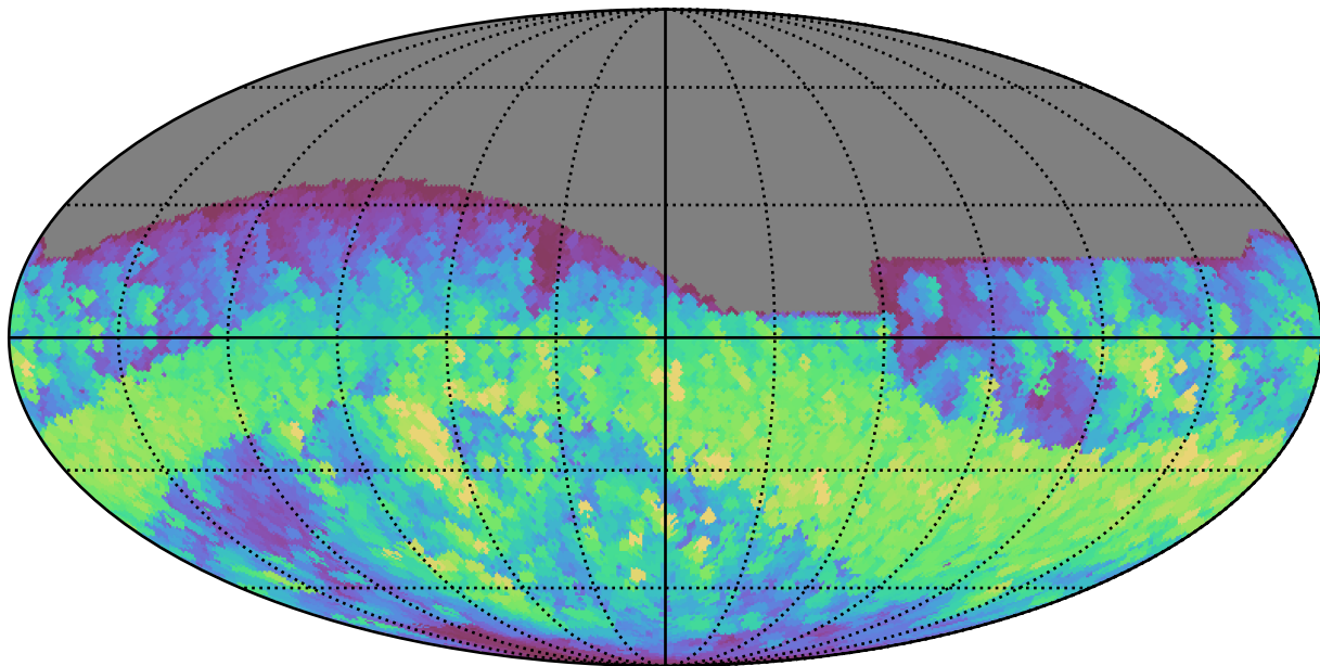
baseline_v3.2_10yrs All sky r band: Max normairmass
