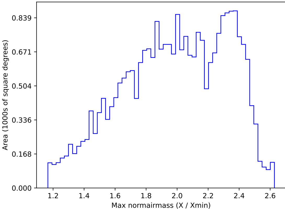
baseline_v3.2_10yrs All sky r band: Max normairmass
