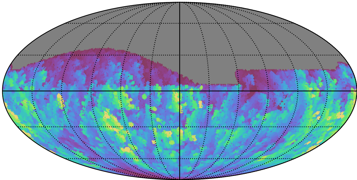
baseline_v3.2_10yrs All sky g band: Max normairmass
