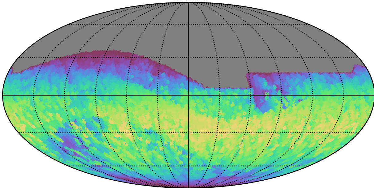
baseline_v3.2_10yrs All sky all bands: Max normairmass
