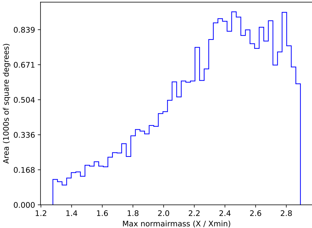
baseline_v3.2_10yrs All sky all bands: Max normairmass
