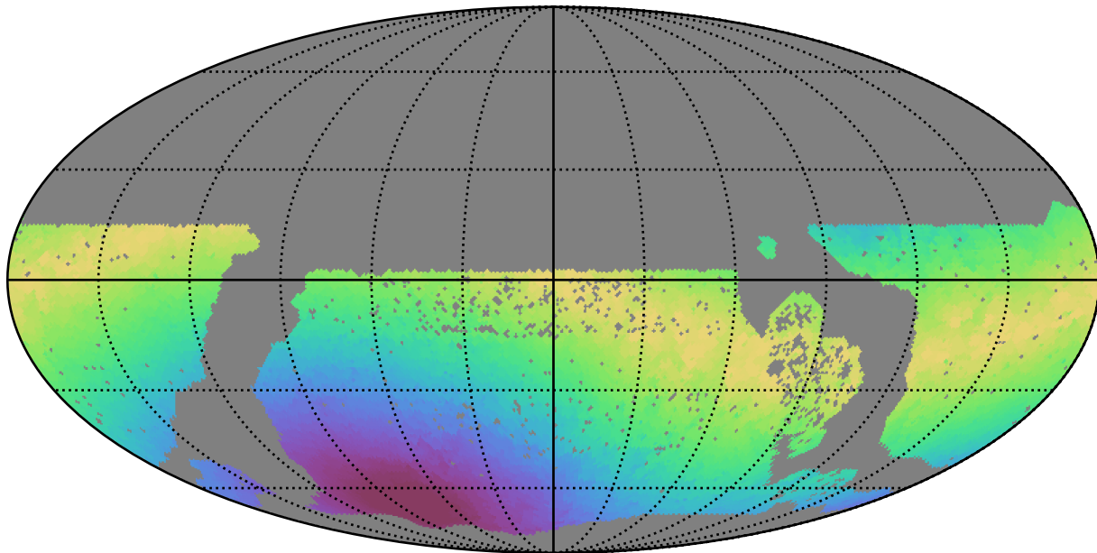
baseline_v3.2_10yrs WFD z band: Max moonDistance
