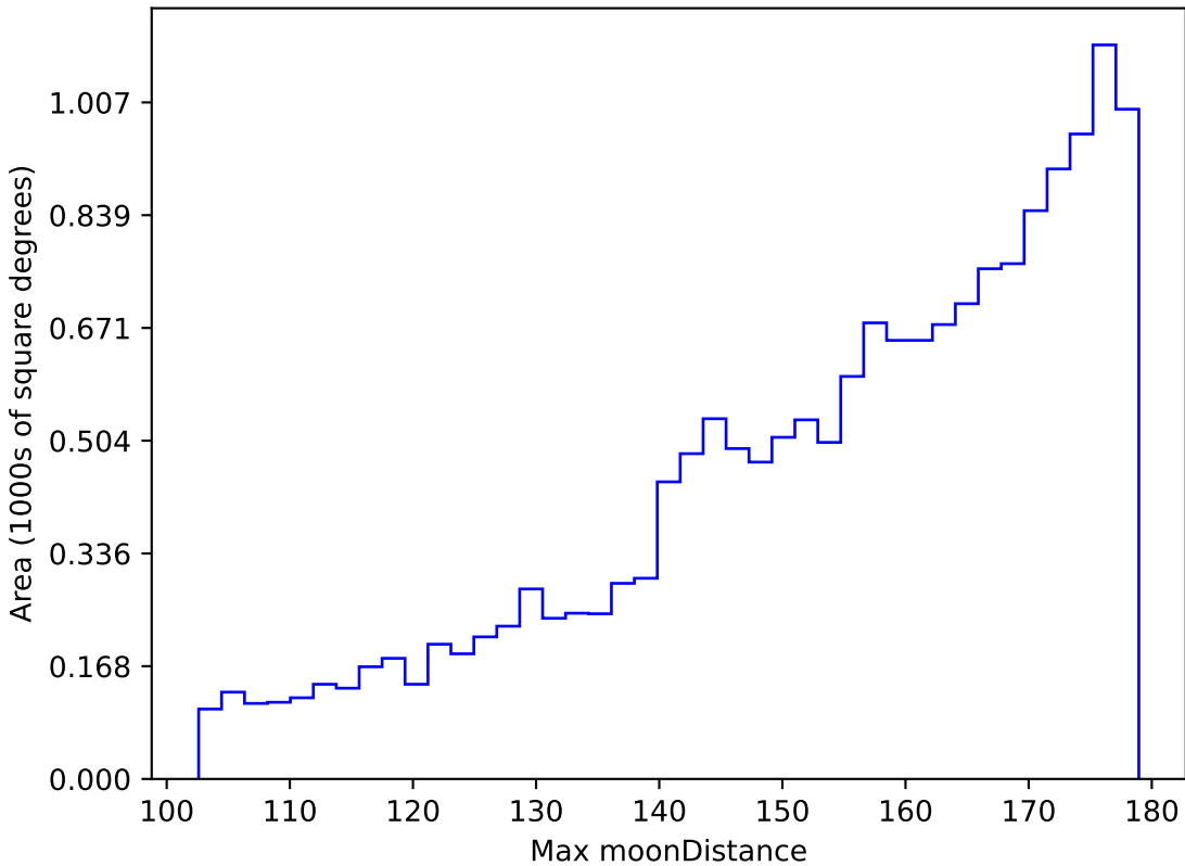
baseline_v3.2_10yrs WFD z band: Max moonDistance
