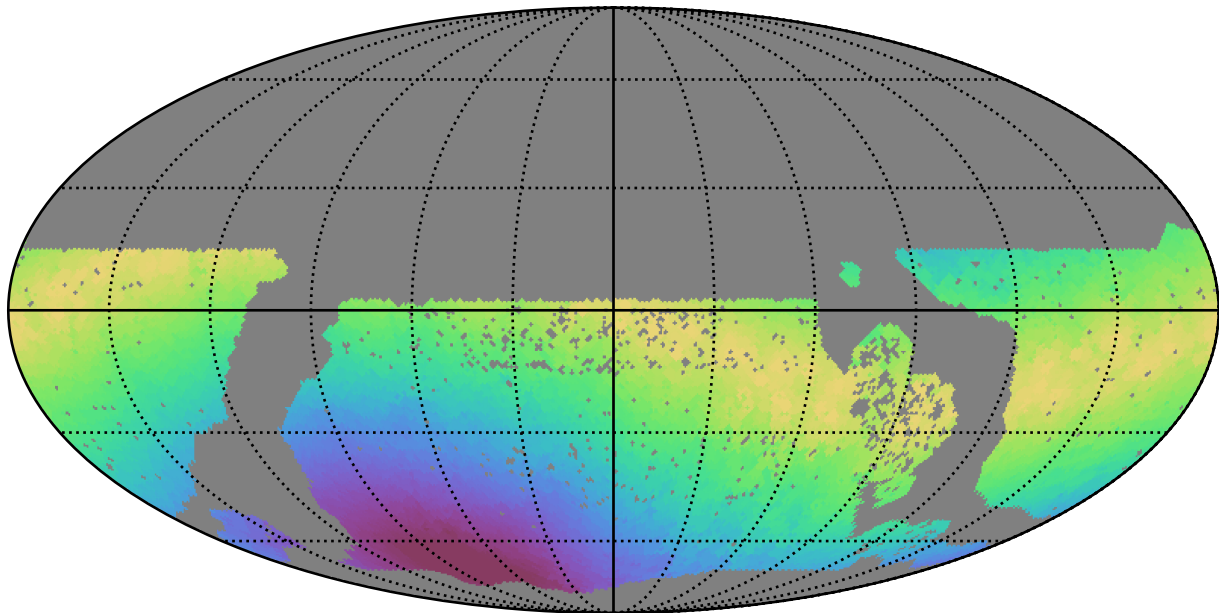
baseline_v3.2_10yrs WFD u band: Max moonDistance
