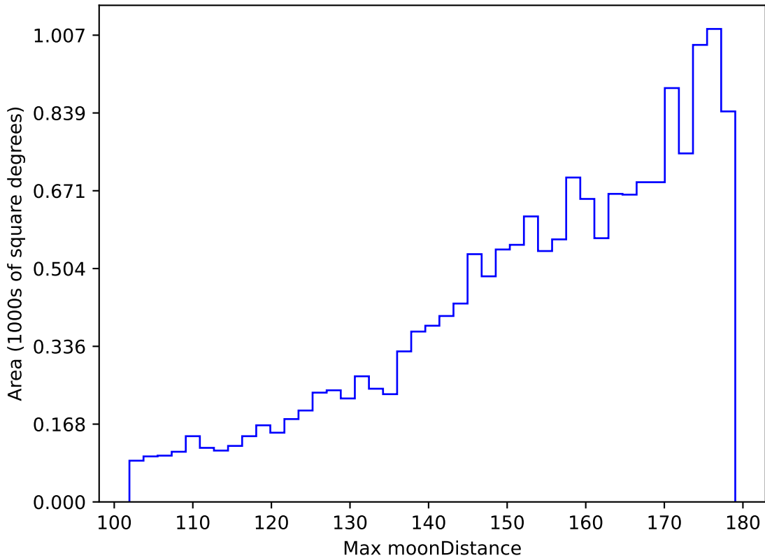
baseline_v3.2_10yrs WFD u band: Max moonDistance
