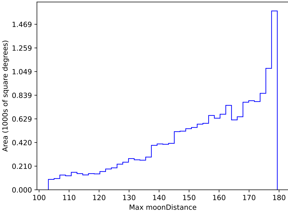
baseline_v3.2_10yrs WFD r band: Max moonDistance
