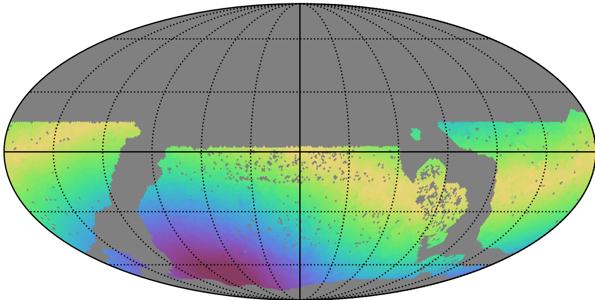
baseline_v3.2_10yrs WFD i band: Max moonDistance
