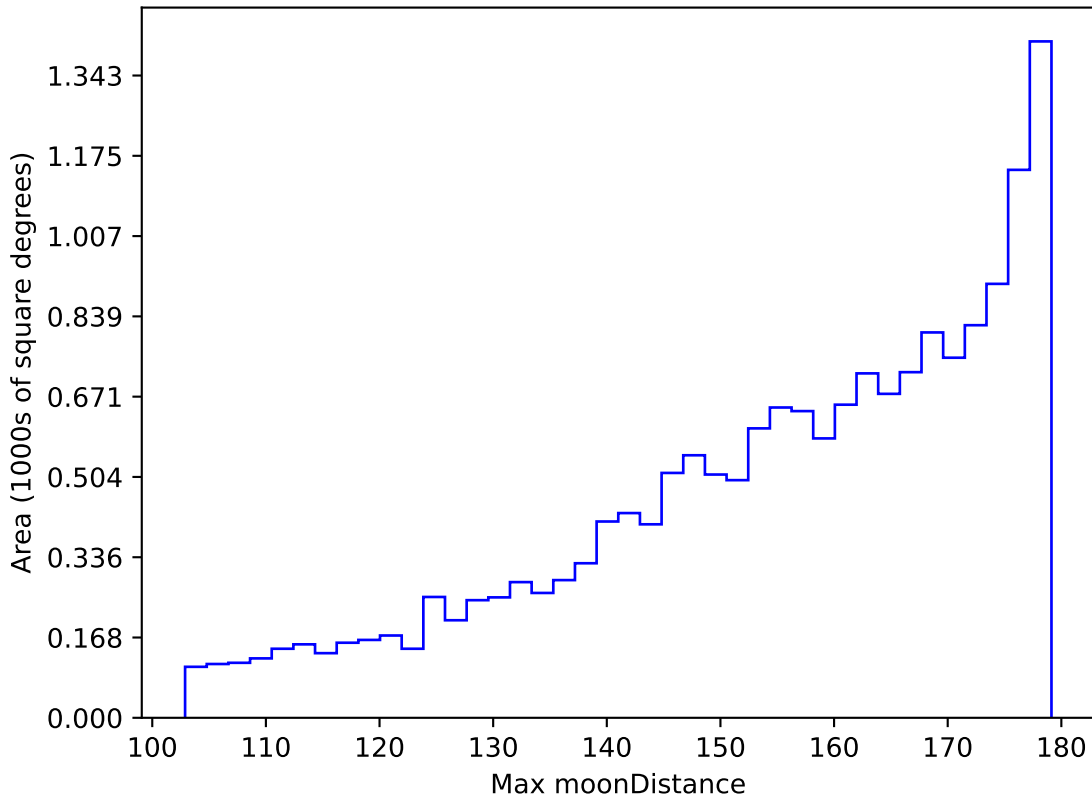
baseline_v3.2_10yrs WFD i band: Max moonDistance
