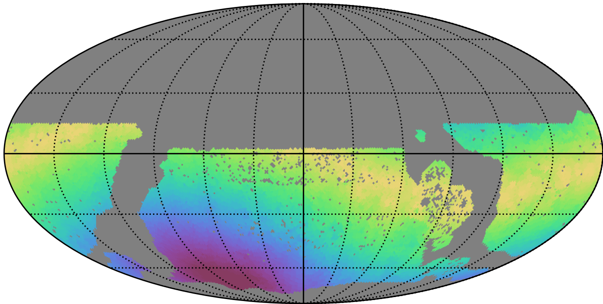
baseline_v3.2_10yrs WFD g band: Max moonDistance
