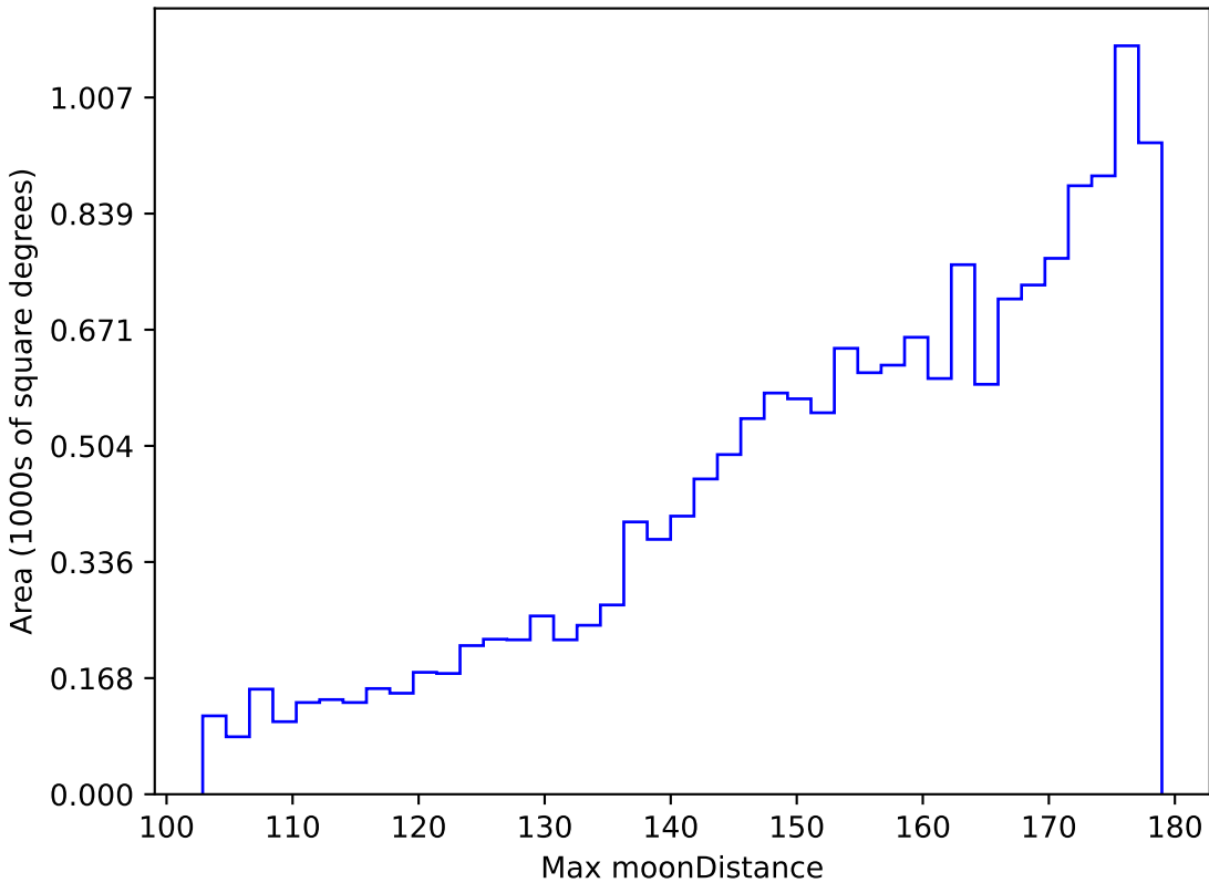
baseline_v3.2_10yrs WFD g band: Max moonDistance
