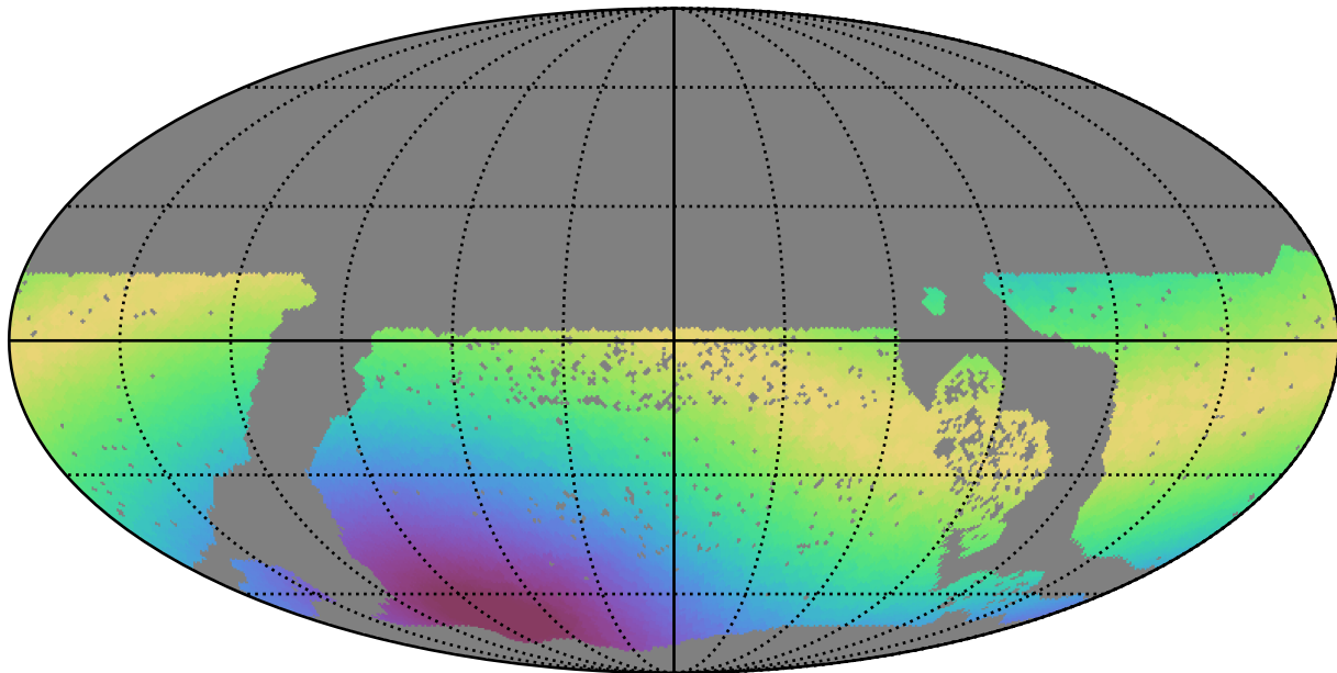
baseline_v3.2_10yrs WFD all bands: Max moonDistance
