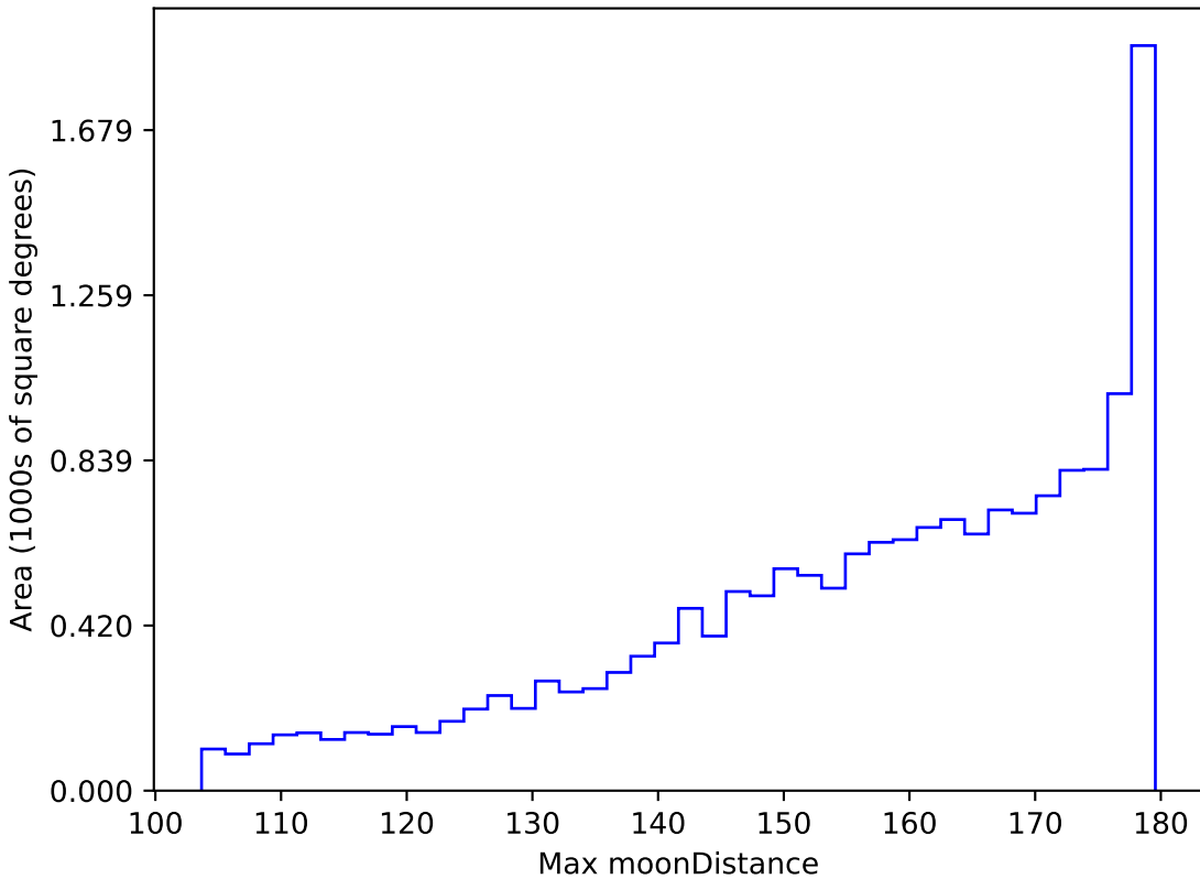
baseline_v3.2_10yrs WFD all bands: Max moonDistance
