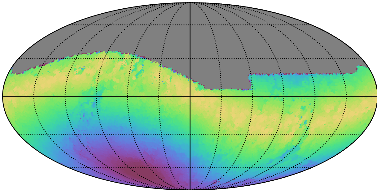
baseline_v3.2_10yrs All sky z band: Max moonDistance
