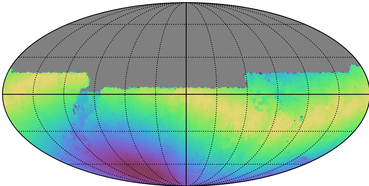
baseline_v3.2_10yrs All sky u band: Max moonDistance
