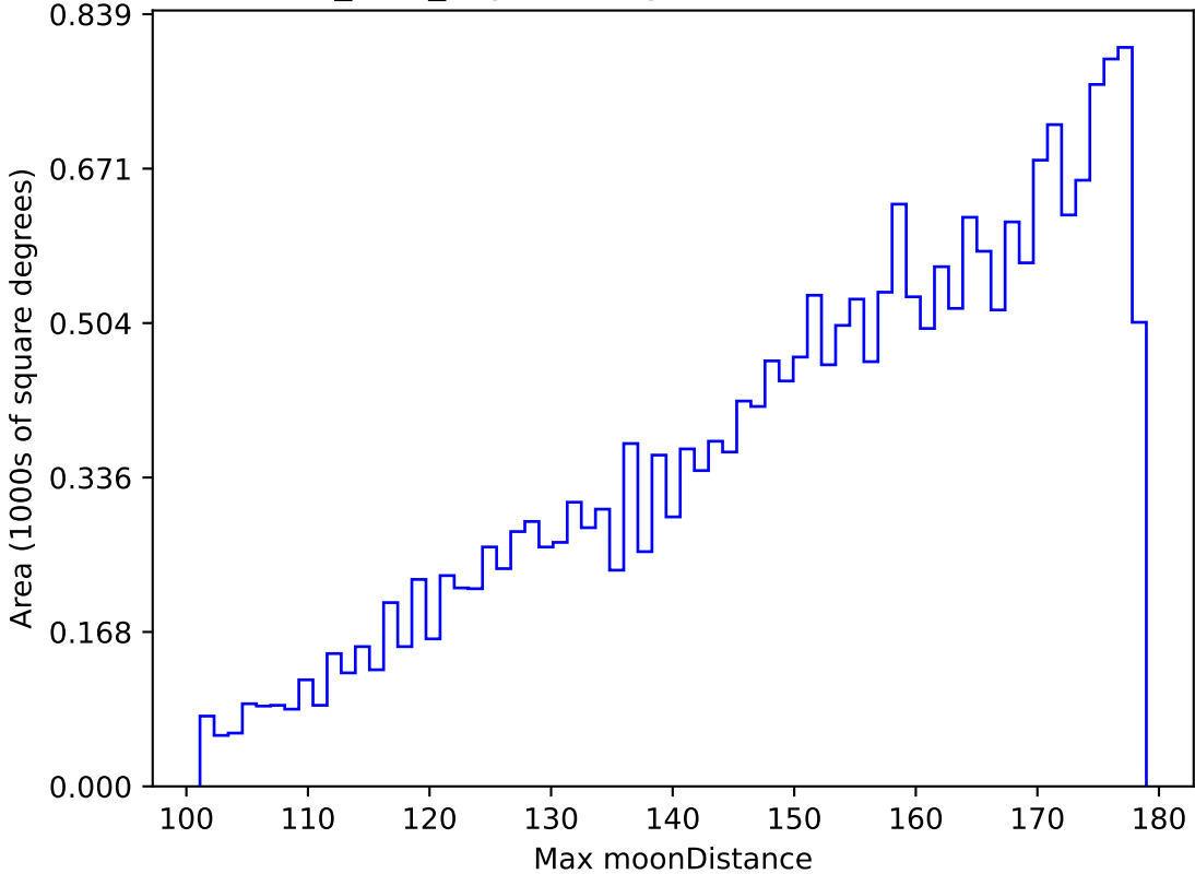
baseline_v3.2_10yrs All sky u band: Max moonDistance
