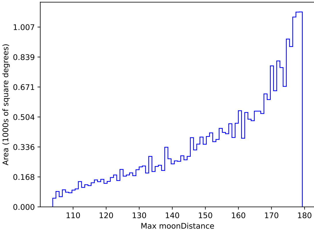
baseline_v3.2_10yrs All sky r band: Max moonDistance
