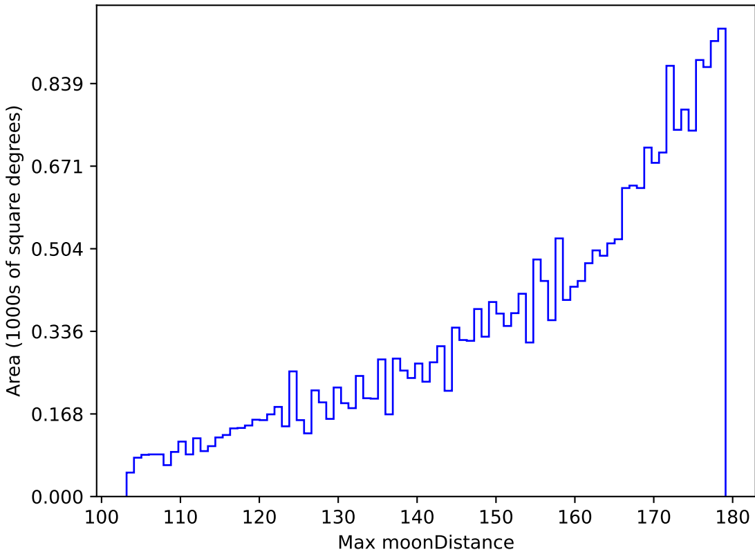
baseline_v3.2_10yrs All sky i band: Max moonDistance
