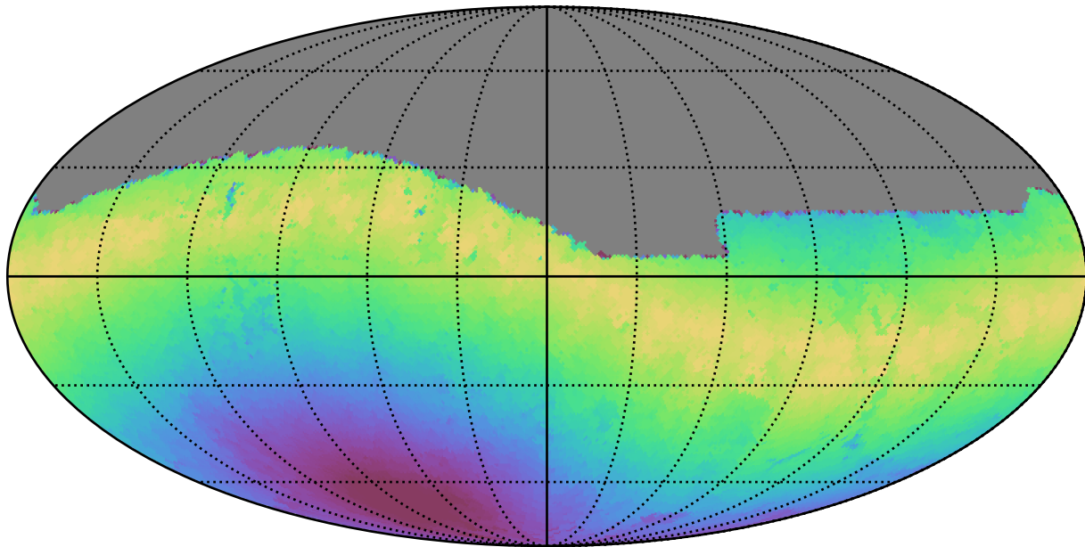
baseline_v3.2_10yrs All sky g band: Max moonDistance
