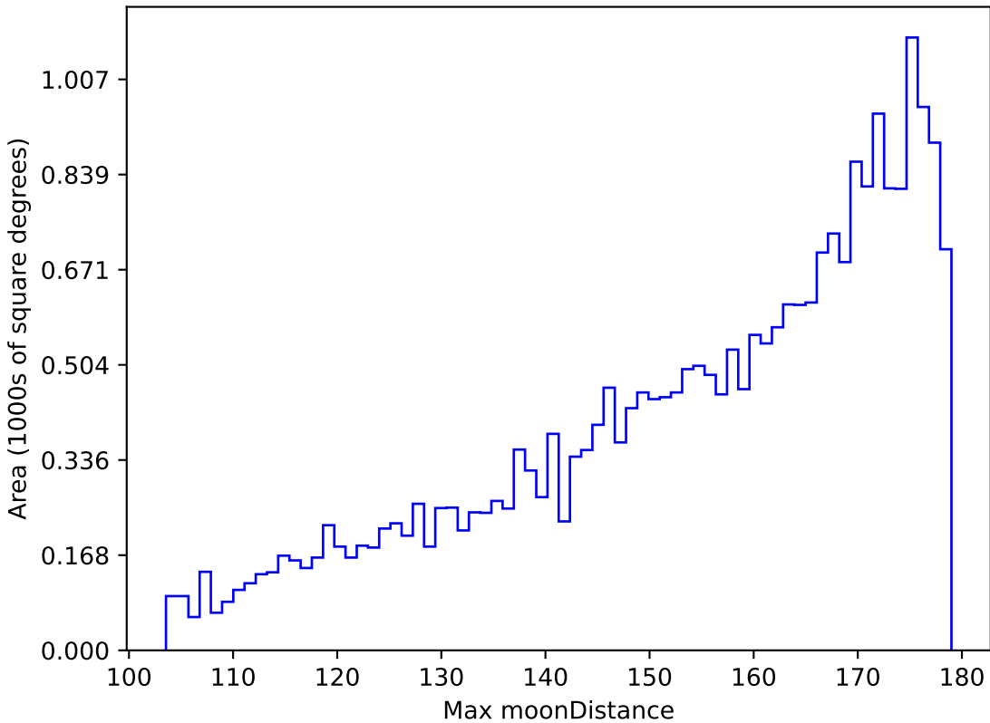
baseline_v3.2_10yrs All sky g band: Max moonDistance
