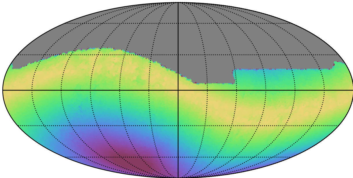
baseline_v3.2_10yrs All sky all bands: Max moonDistance
