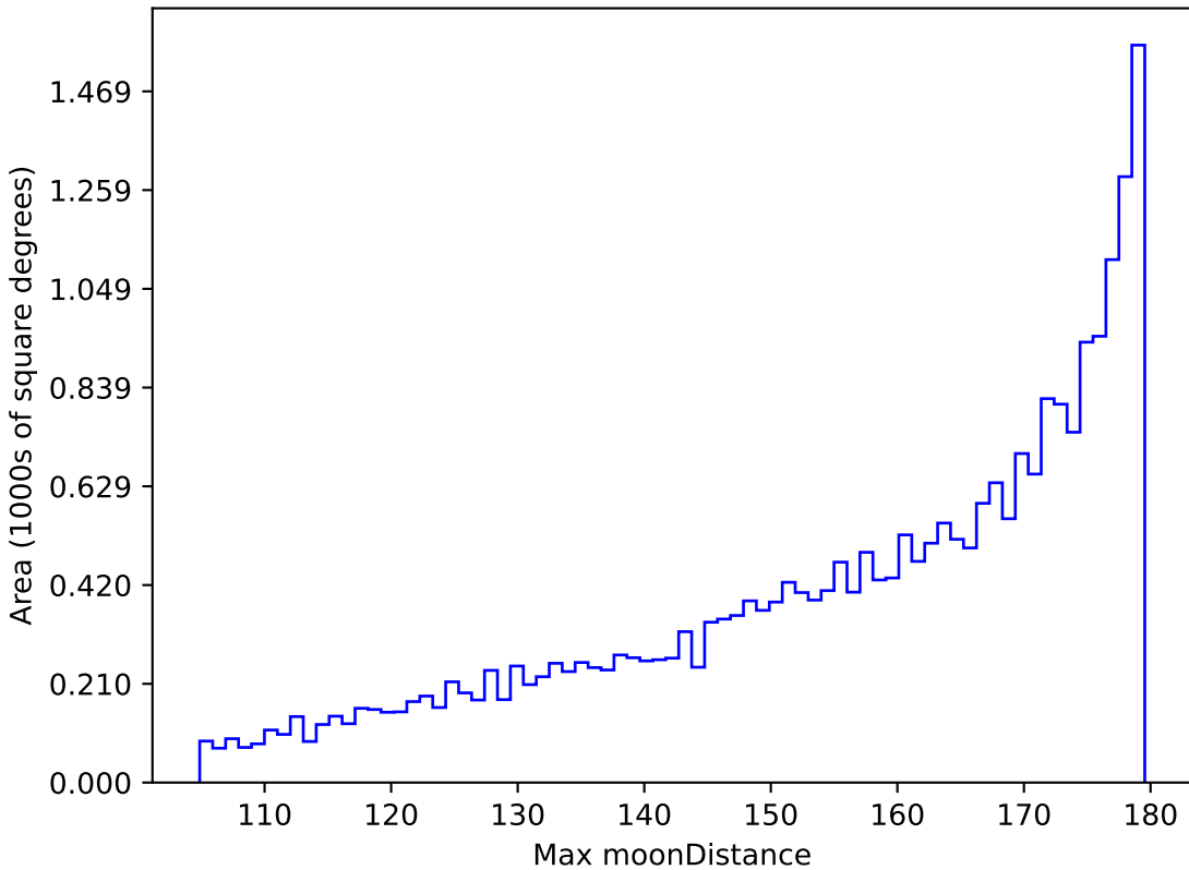
baseline_v3.2_10yrs All sky all bands: Max moonDistance
