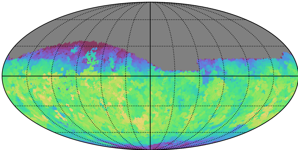
baseline_v3.2_10yrs Yr 1 z band: Max fiveSigmaDepth
