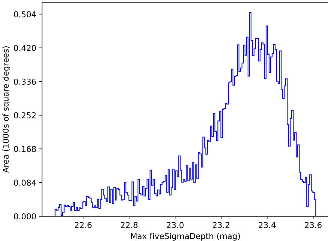
baseline_v3.2_10yrs Yr 1 z band: Max fiveSigmaDepth
