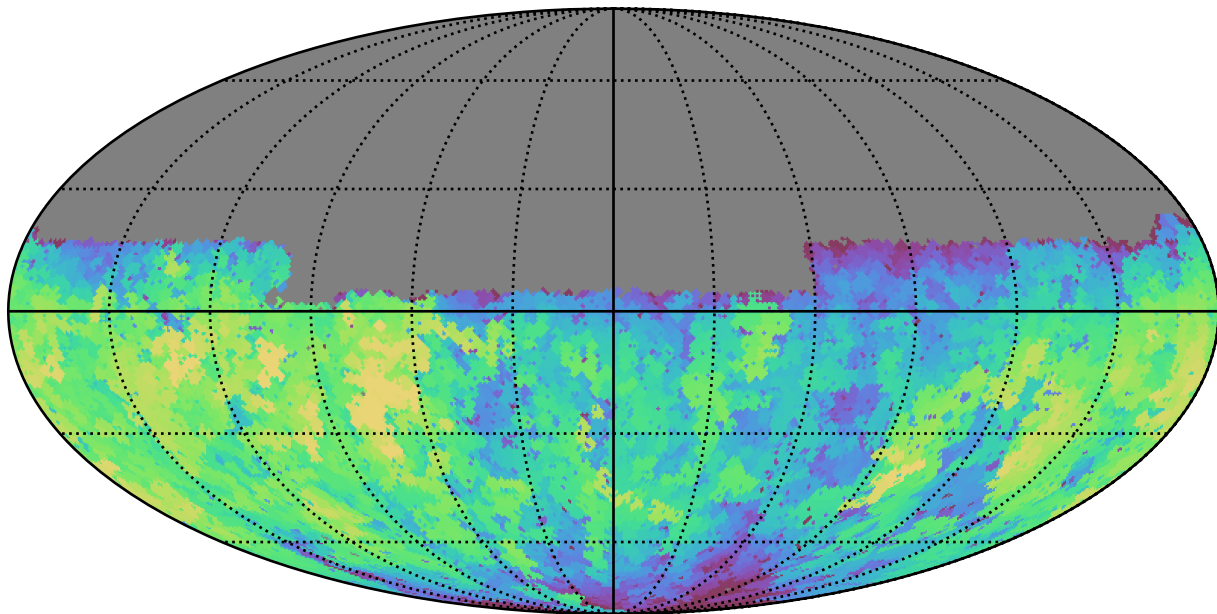
baseline_v3.2_10yrs Yr 1 u band: Max fiveSigmaDepth
