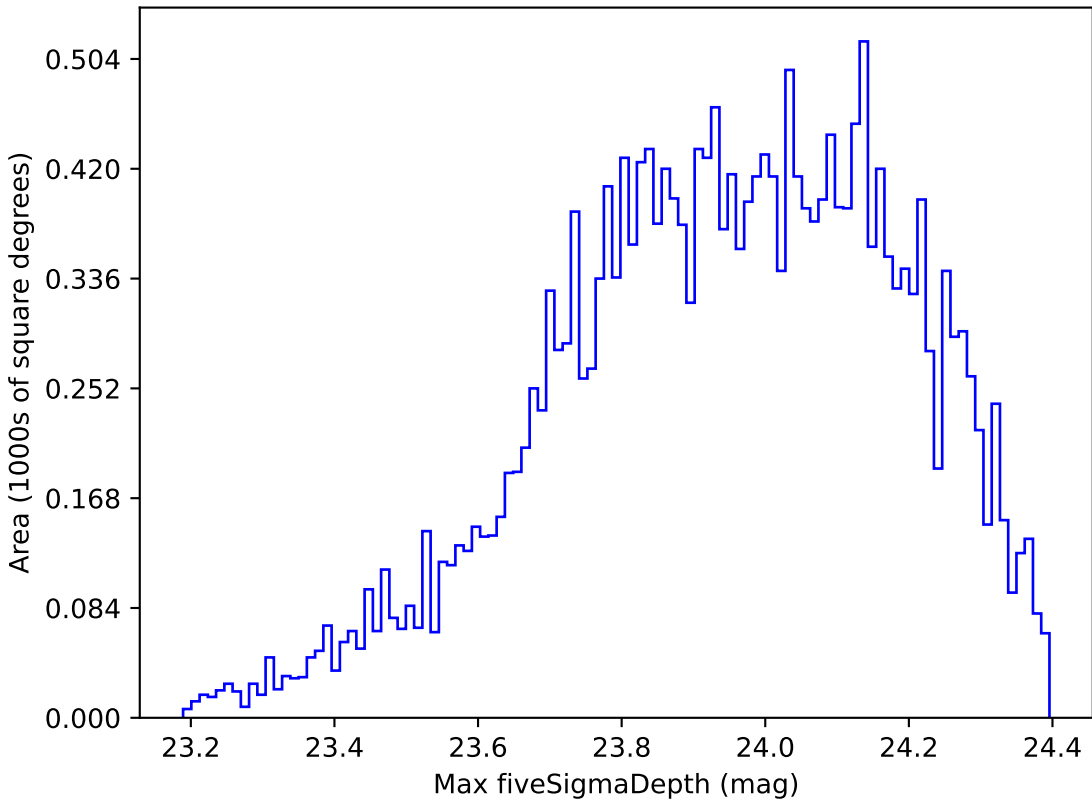
baseline_v3.2_10yrs Yr 1 u band: Max fiveSigmaDepth
