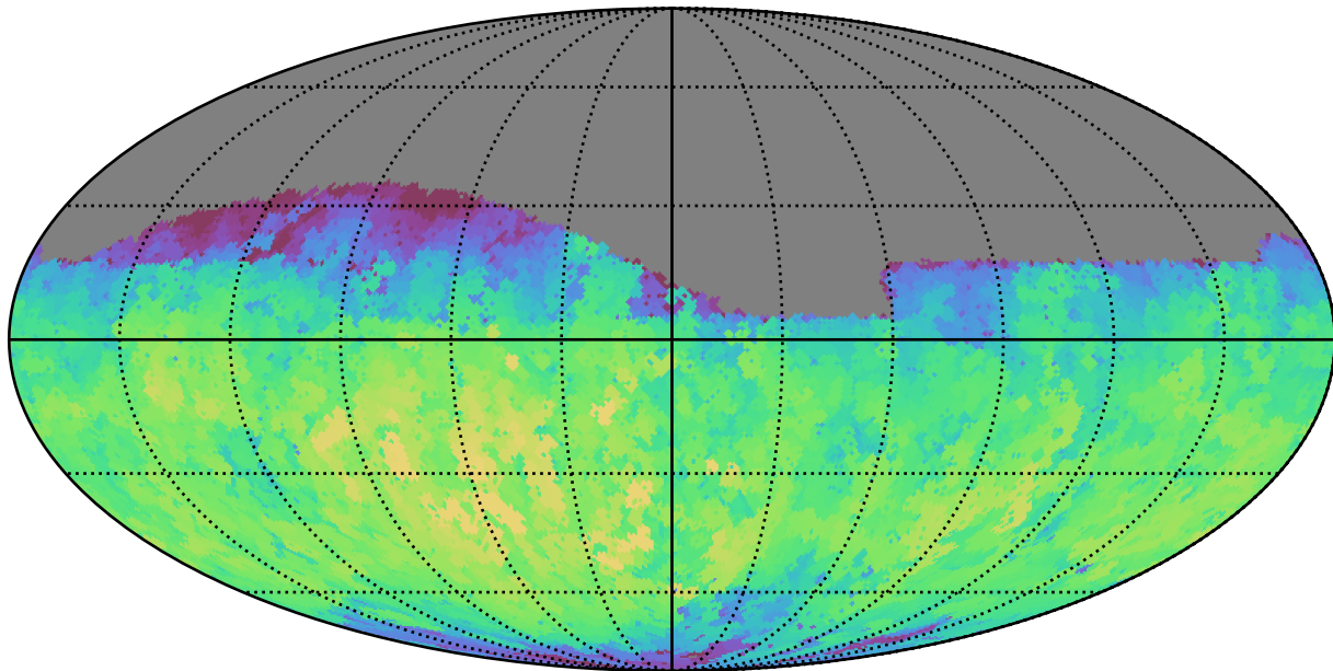
baseline_v3.2_10yrs Yr 1 r band: Max fiveSigmaDepth
