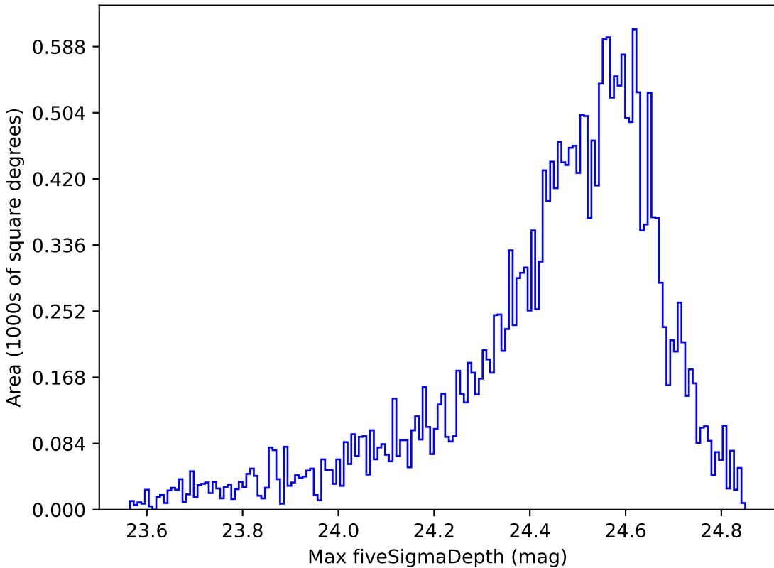
baseline_v3.2_10yrs Yr 1 r band: Max fiveSigmaDepth
