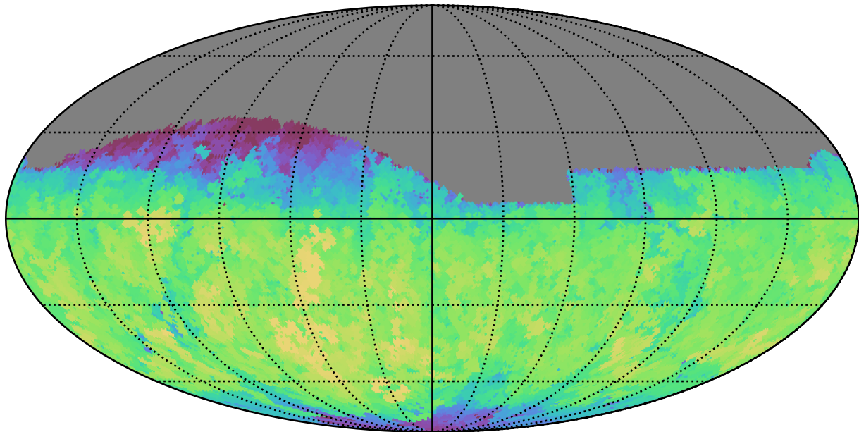
baseline_v3.2_10yrs Yr 1 i band: Max fiveSigmaDepth
