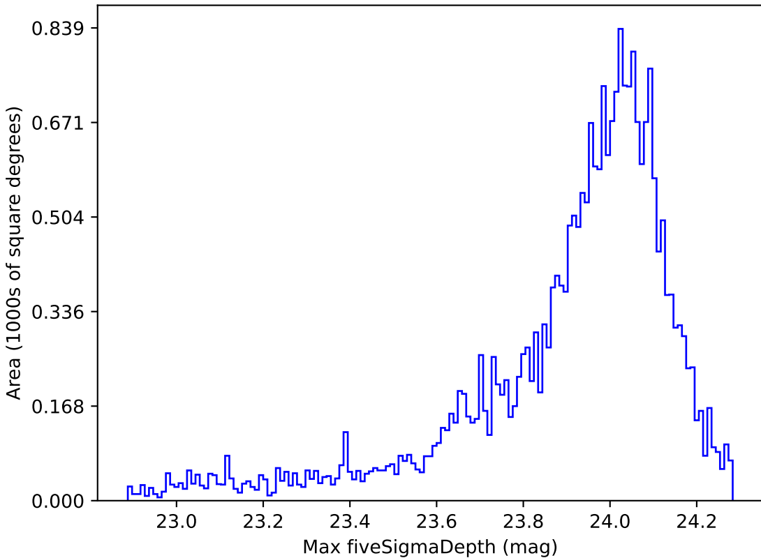
baseline_v3.2_10yrs Yr 1 i band: Max fiveSigmaDepth
