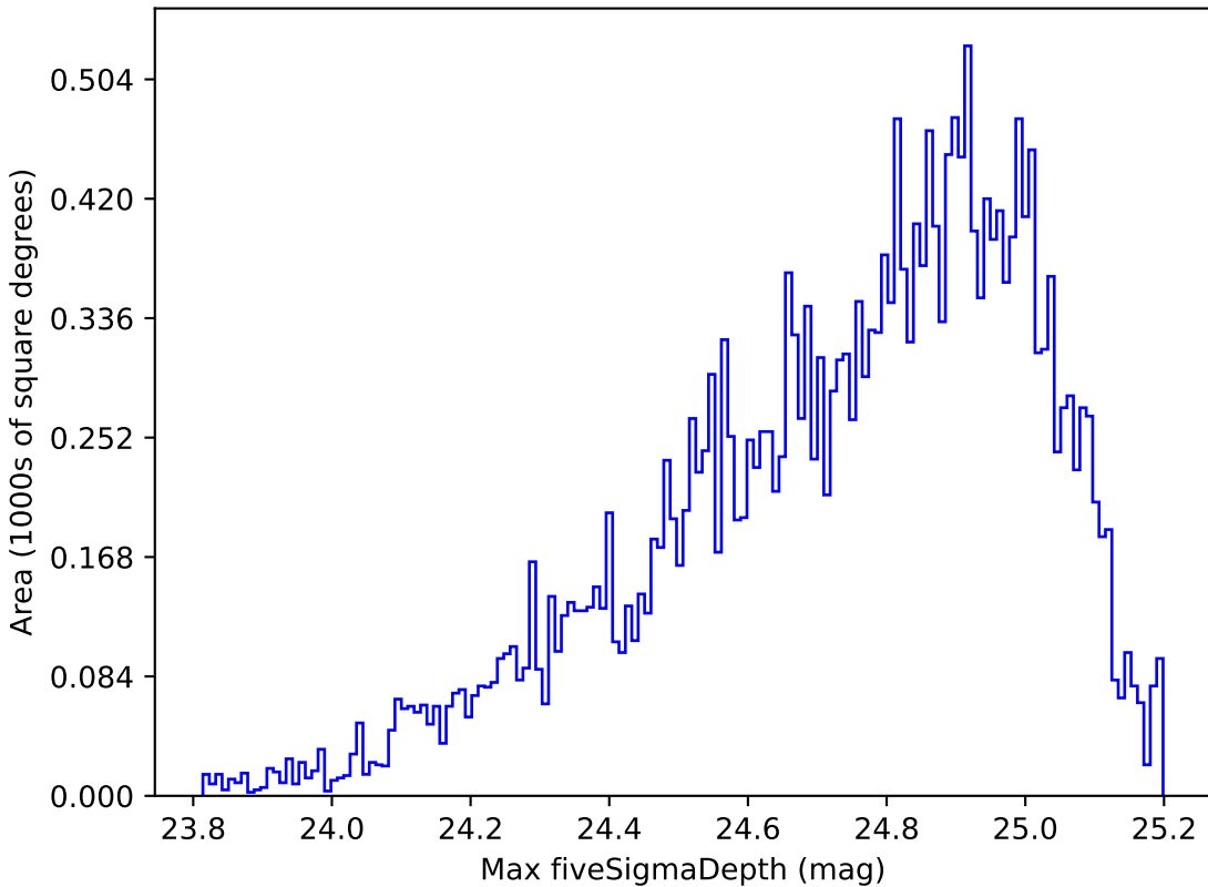
baseline_v3.2_10yrs Yr 1 g band: Max fiveSigmaDepth
