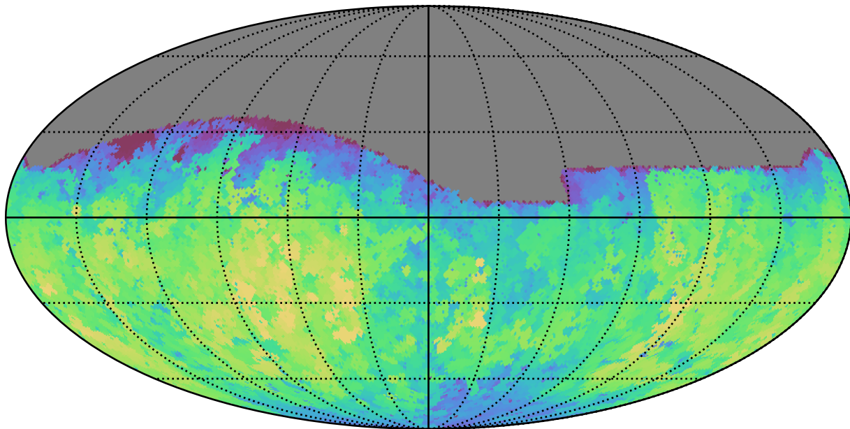
baseline_v3.2_10yrs Yr 1 all bands: Max fiveSigmaDepth
