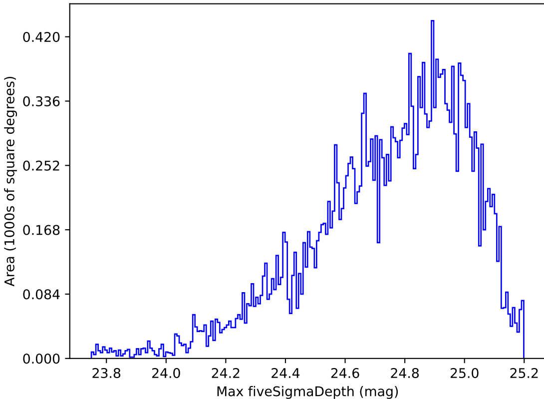
baseline_v3.2_10yrs Yr 1 all bands: Max fiveSigmaDepth
